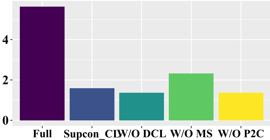
Calmar Ratio
